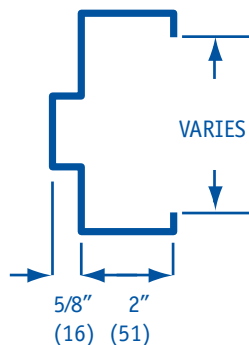
TYPICAL SECTION
